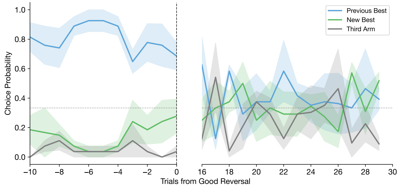
Good Reversal-Aligned Choices (mean \pm se across subjects | n=3 subjects, n=20 reversals) (Skipping first 15 trials post-reversal)
